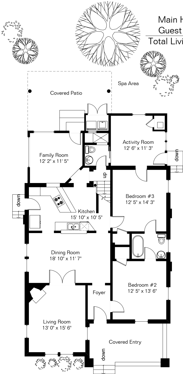
Main Level
